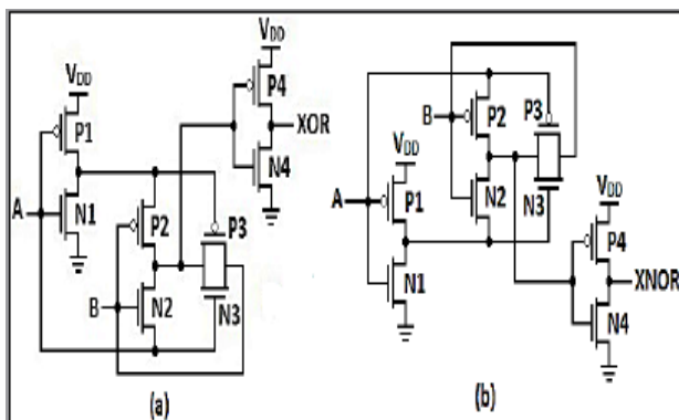
Fig.2. XOR/XNOR transmission gate
