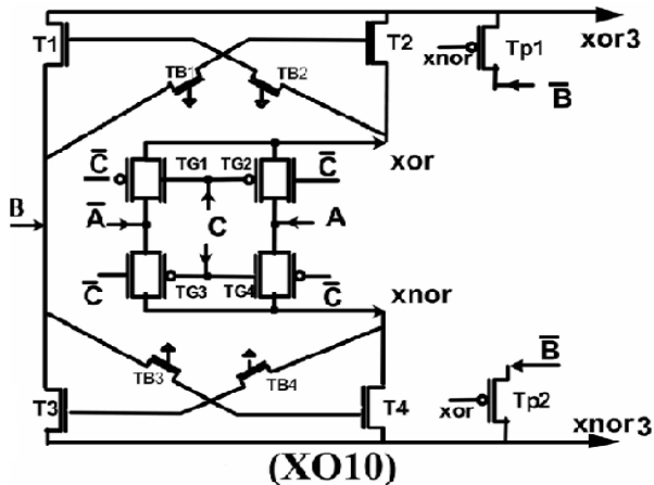
Fig.3. Three-input XOR/XNOR circuits XO4, XO7, and XO10
