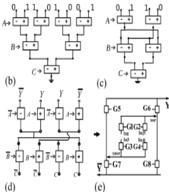
Fig.1. (a) SCDM process for designing efficient three-input XOR/XNORs. (b) BDT representation of three-input XOR/XNOR function. (c) Applying reduction rules. (d) Substitution and disjointing. (e) EBC
