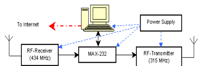
Fig.4. Block diagram of the client
