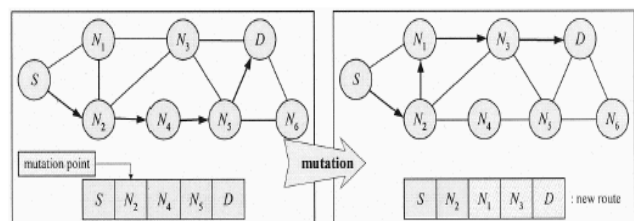
Fig.9. Mutation Procedure
