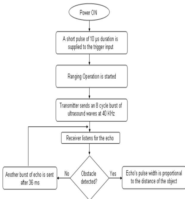
Fig.7. Flow chart for distance measurement
