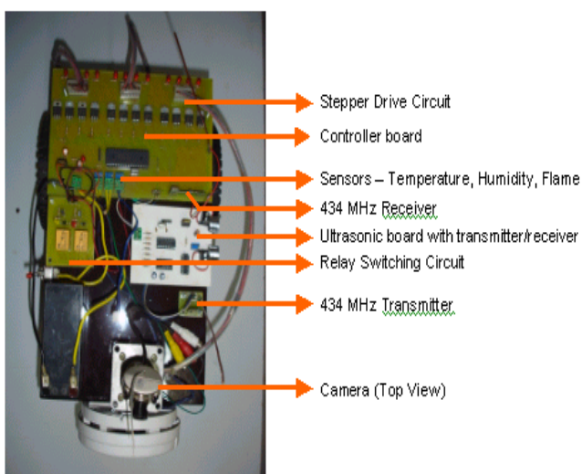
Fig.1. Top View of Soft-i-Robot
