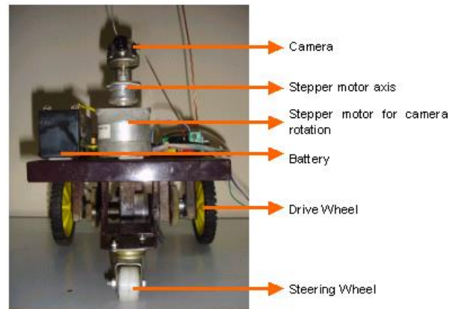
Fig.2. Front View of Soft-i-Robot
