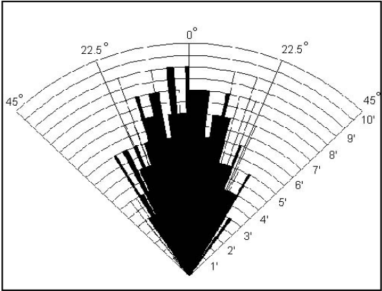
Fig.11. Beam Pattern of the Ultrasonic wave
