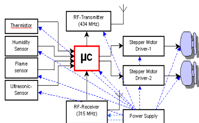
Fig.3. Block diagram of the control board
