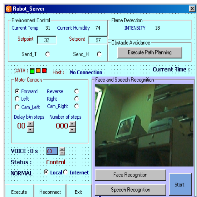
Fig.13. Front Panel of Server
