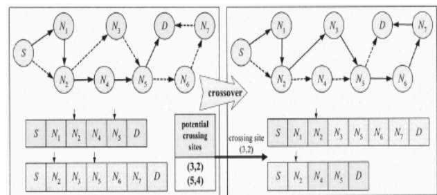
Fig.8. Crossover Procedure
