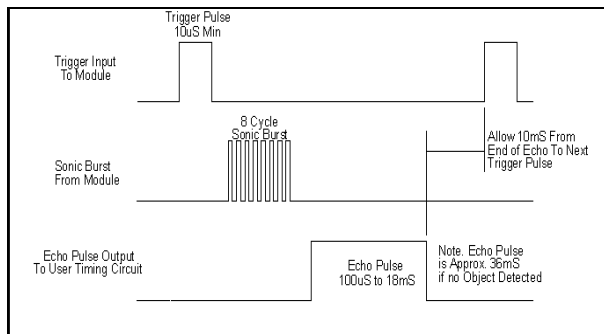
Fig.12. SRF04 Timing Diagram
