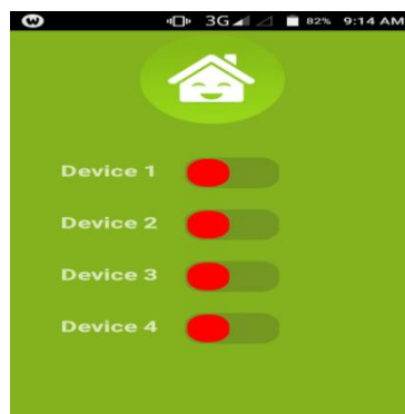
Figure 2 Android applications
